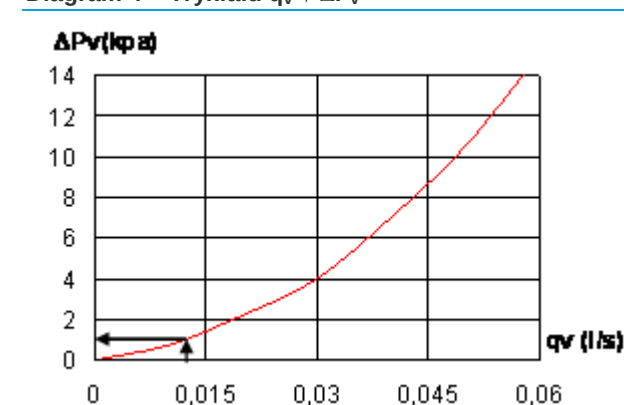
Diagram 4 – Trykfald q_v \rightarrow \Delta P_v
